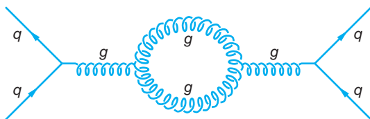
FIGURE 12-27 Feynman diagram of a quark emitting a gluon, which then creates two gluons—a gluon loop or bubble—that recombine, the resulting gluon being absorbed by another quark.
